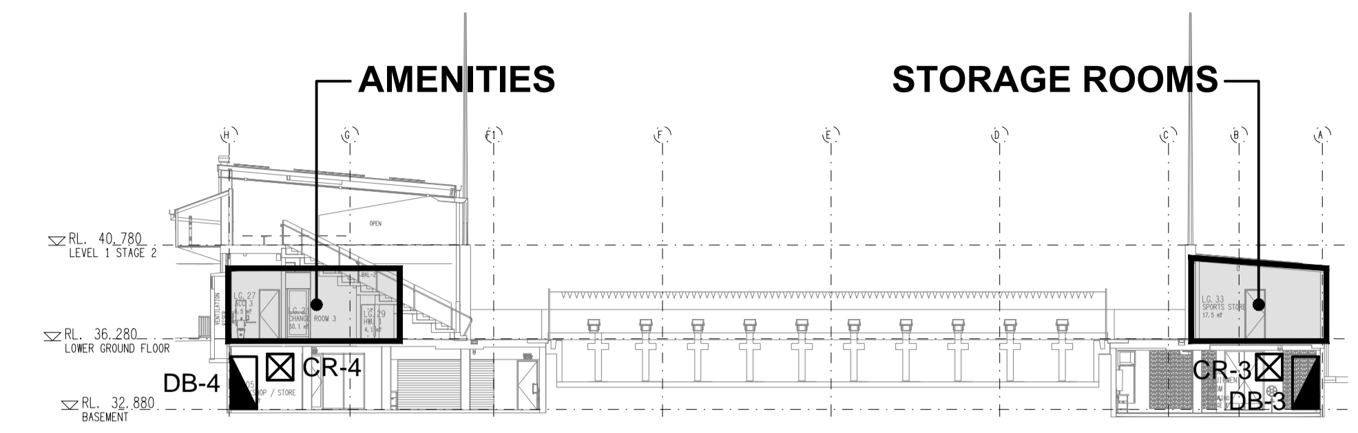
SECTION A LOWER GROUND STORAGE & AMENITIES SCALE 1:250
