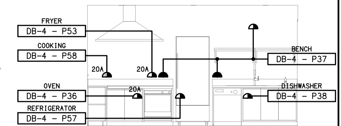
DETAIL C STORE ROOM BENCH ELEVATION 3 SCALE 1:50
