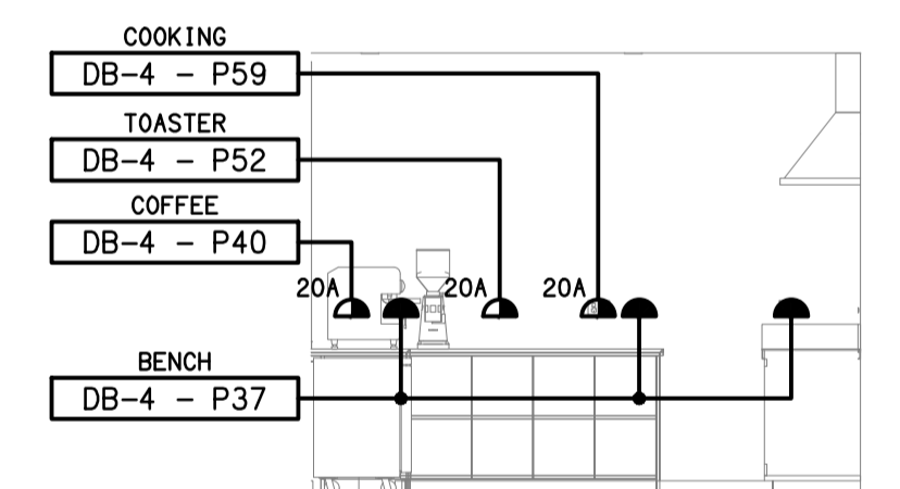
DETAIL B STORE ROOM BENCH ELEVATION 2 SCALE 1:50
